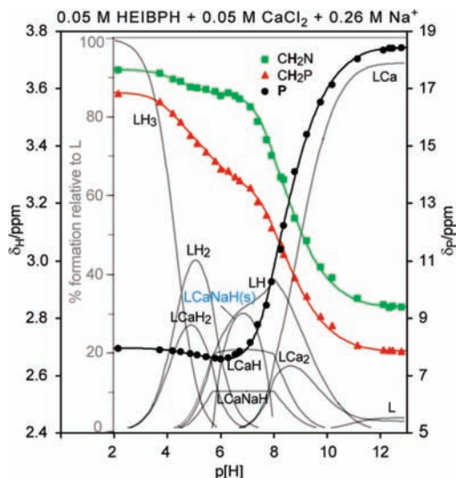
Figure 4. Single-sample ^{31}\text{P} and ^1\text{H} NMR titration curves \delta versus \text{p}[\text{H}] of solution containing 0.05 M HEIBPH (1), 0.05 M \text{CaCl}_2 , and 0.26 M \text{Na}^+ . The solid lines between the experimental values are drawn by joining calculated values, obtained using the simulated equilibrium constants and the supposed individual chemical shifts. Gray lines show the calculated species distribution (charges of species are omitted).
